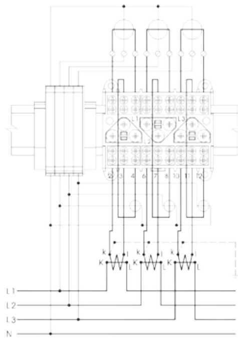
Connection of terminal board ZS4 / ZS4-M with connected electricity meter and control measuring devices
