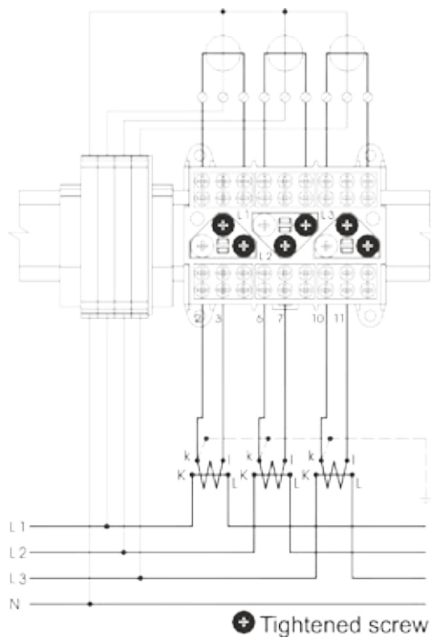
Connection of terminal board ZS4 / ZS4-M with connected electricity meter
